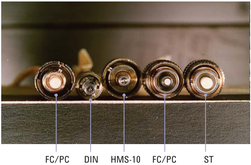
Connector types showing various constructions, e.g. metallic, ceramic, etc.
