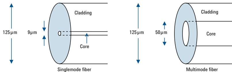
Figure 1. Optical fibers
