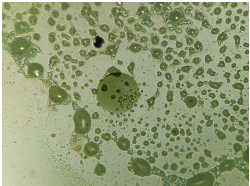
Ceramic ferrule showing RI liquid contamination
